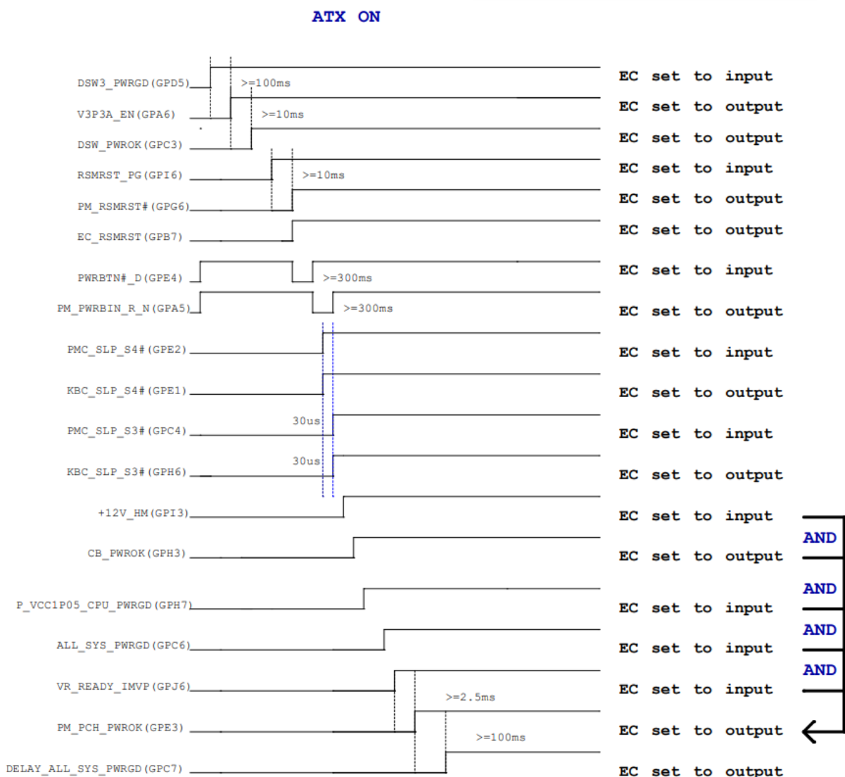
Figure 17 B658VGL ATX Mode power sequence
