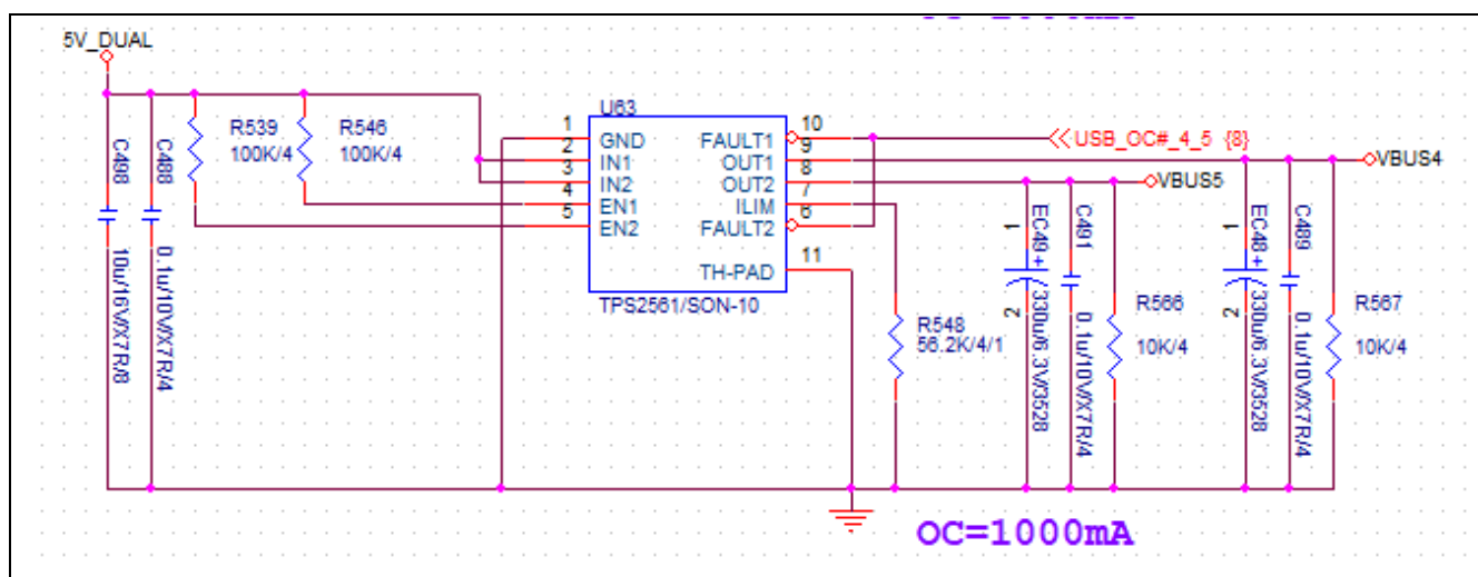
Figure 8 USB 2.0/3.0 Reference schematic 2
