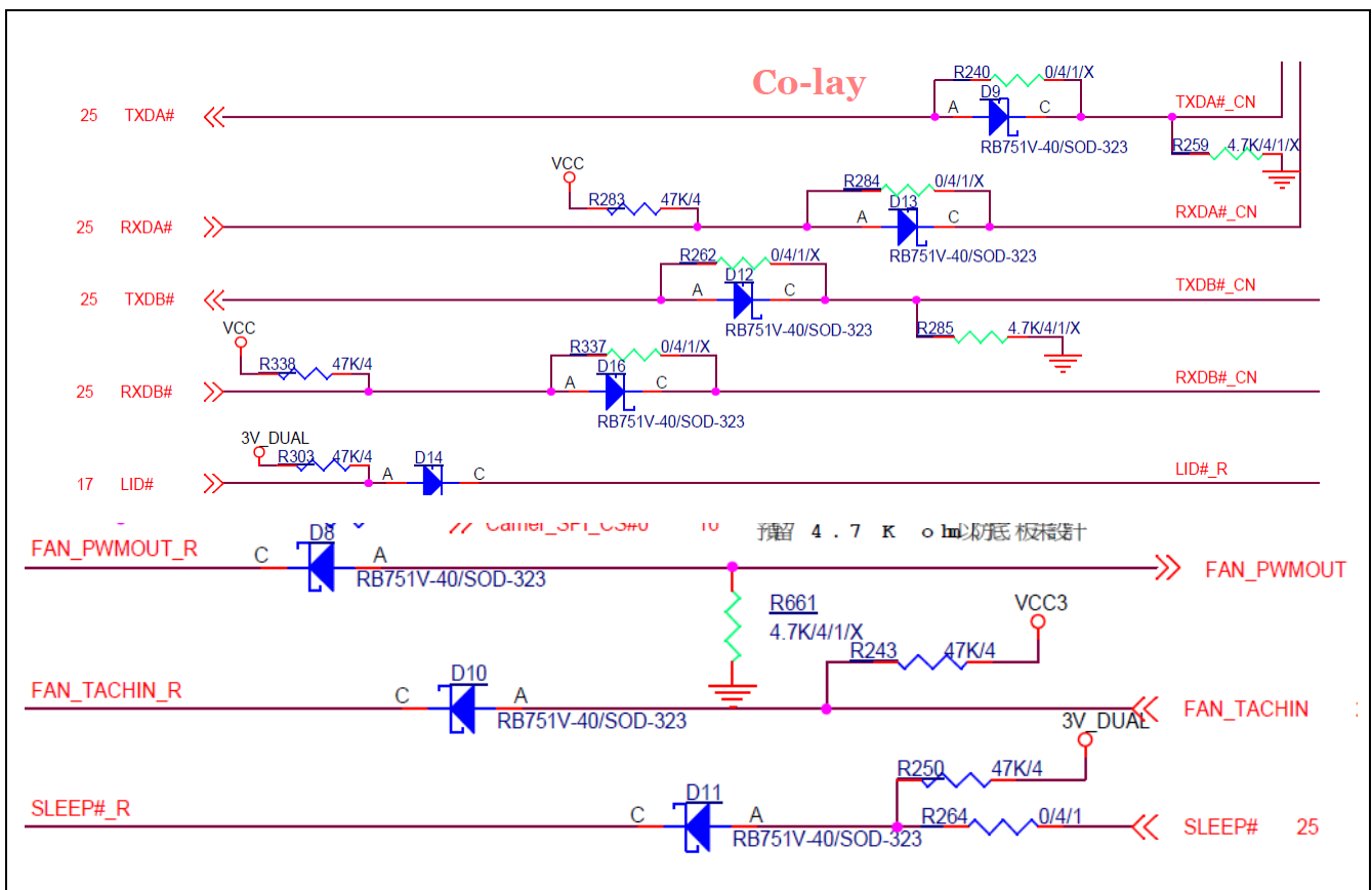
Figure 21 Circuit protection on Module
