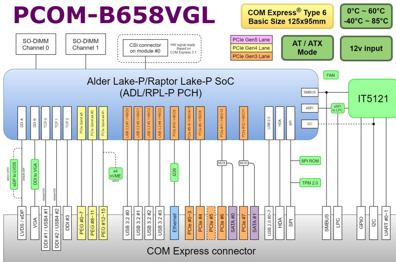
Figure 1 PCOM-B658VGL Block Diagram
