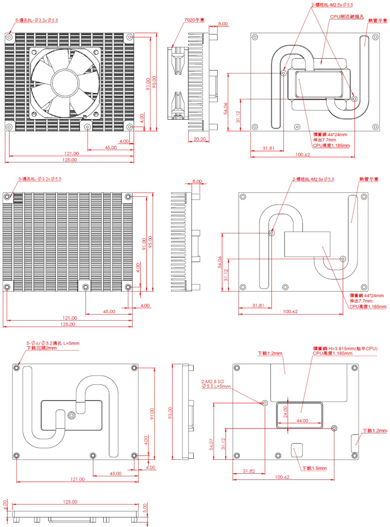
Figure 20 PCOM-B658VGL cooler / heatsink / heatspreader dimension
