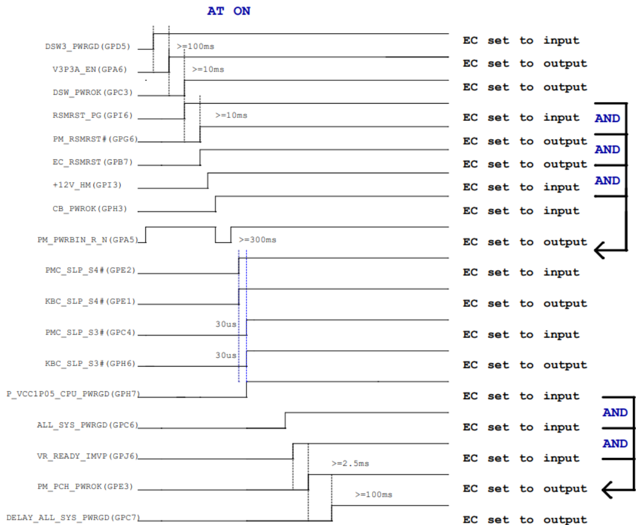
Figure 18 B658VGL AT Mode power sequence
