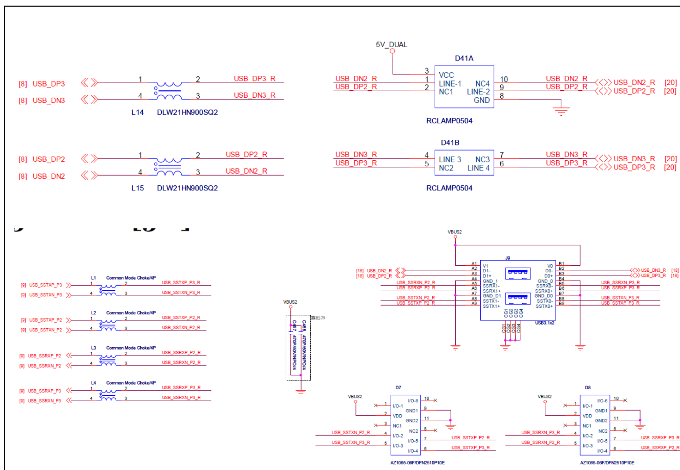
Figure 7 USB 2.0 / 3.0 Reference schematic 1
