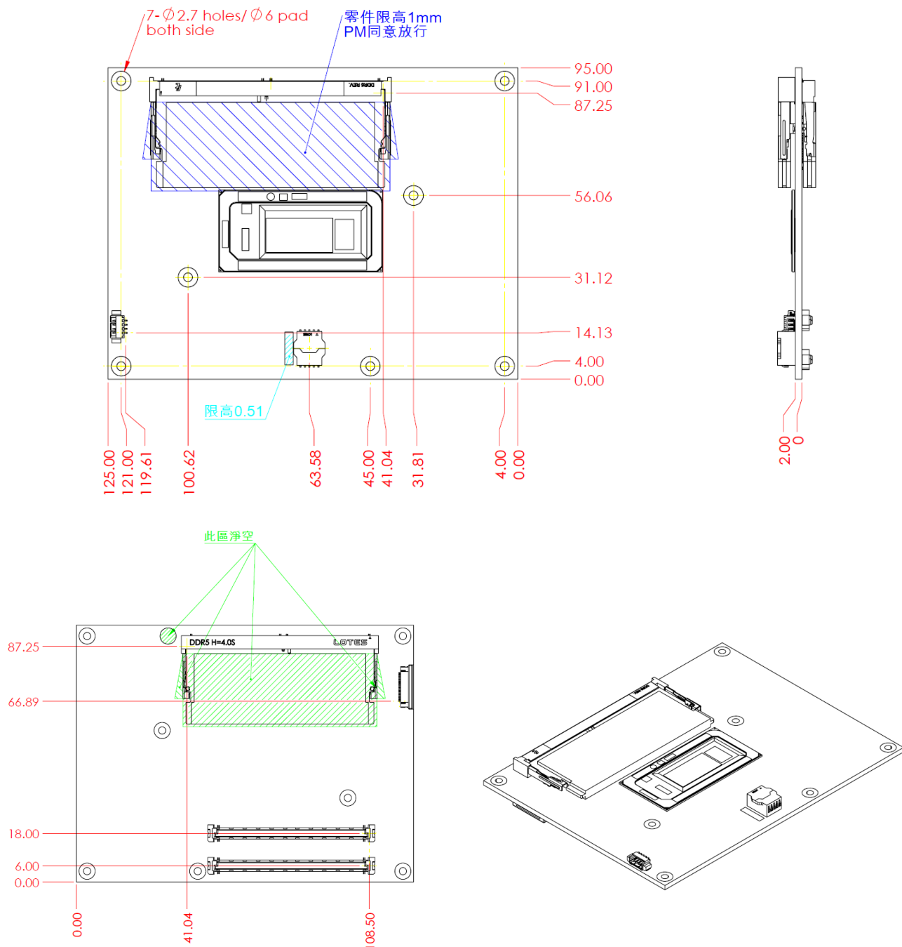
Figure 19 PCOM-B658VGL Dimension – TOP & Bottom
