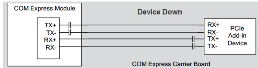
Figure 2 PCIE AC Coupling Capacitor - Device Down
