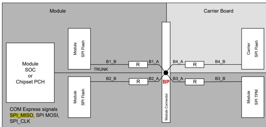
Figure 5.13: COM Express BOOT SPI Topology – Data and Clock lines
