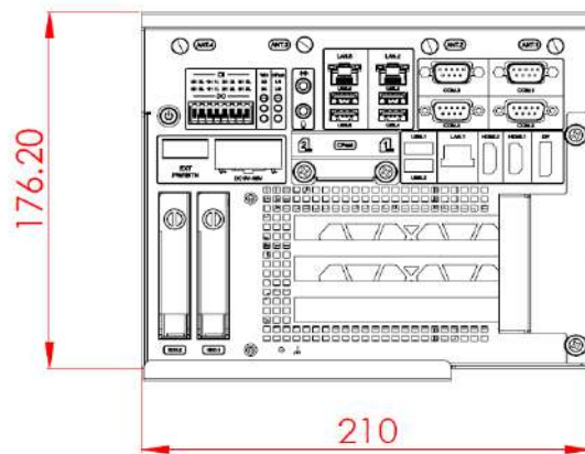
Front view of the WEBS-85H2 system
