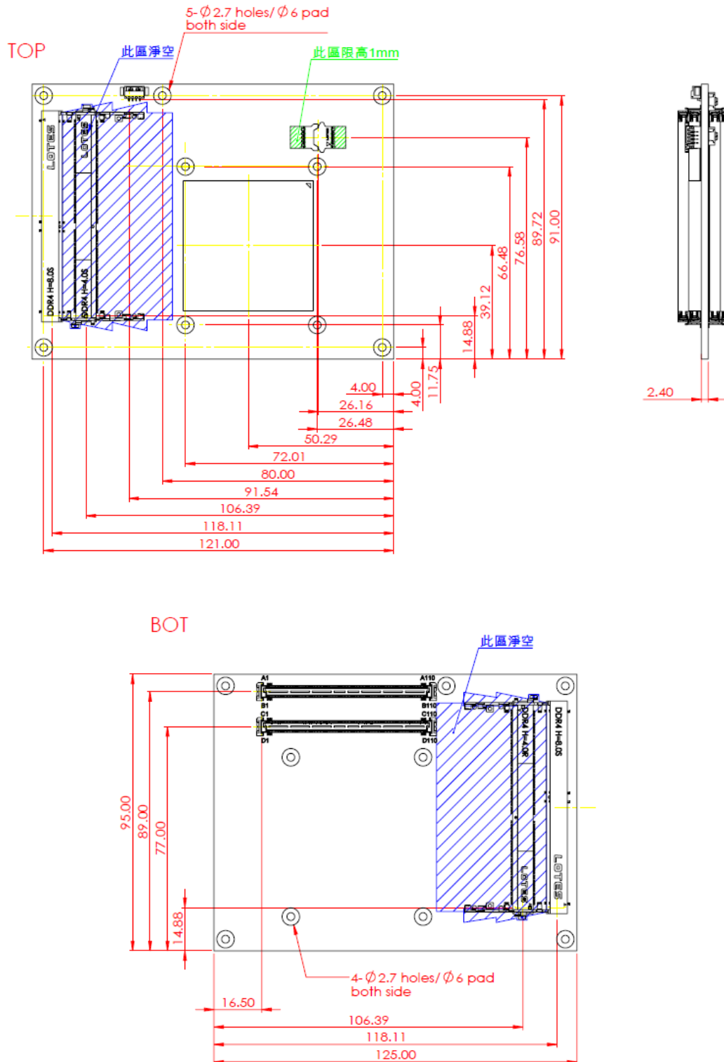
Figure 13 Mechanical – Top, Side and Bottom View
