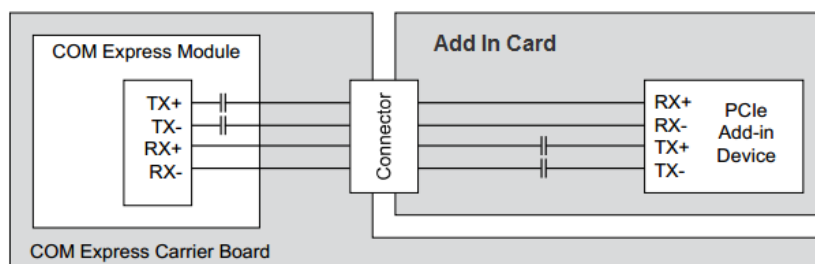
Figure 4 PCIE AC Coupling Capacitor - Add In Card (From PICMG COM Express Carrier Board Design Guide)
