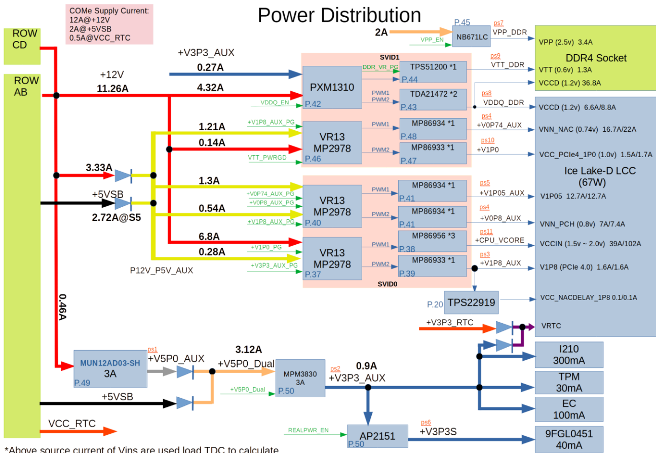
Figure 12 Power Distribution
